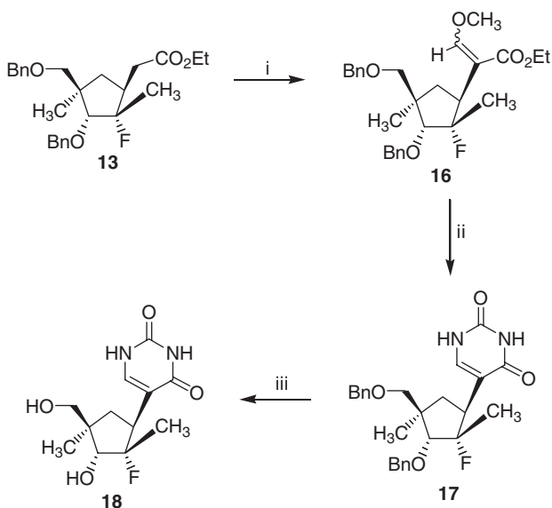
SCHEME 3 Synthesis of target 2'-fluorinated isouracil nucleoside analogue. Reagents: i) (a) LDA/THF, HCOEt; (b) MeI, DMF; ii) \text{NH}_2\text{CONH}_2 , t-BuOK, THF; iii) Pd black, 5% \text{HCO}_2\text{H} in MeOH, reflux overnight.
