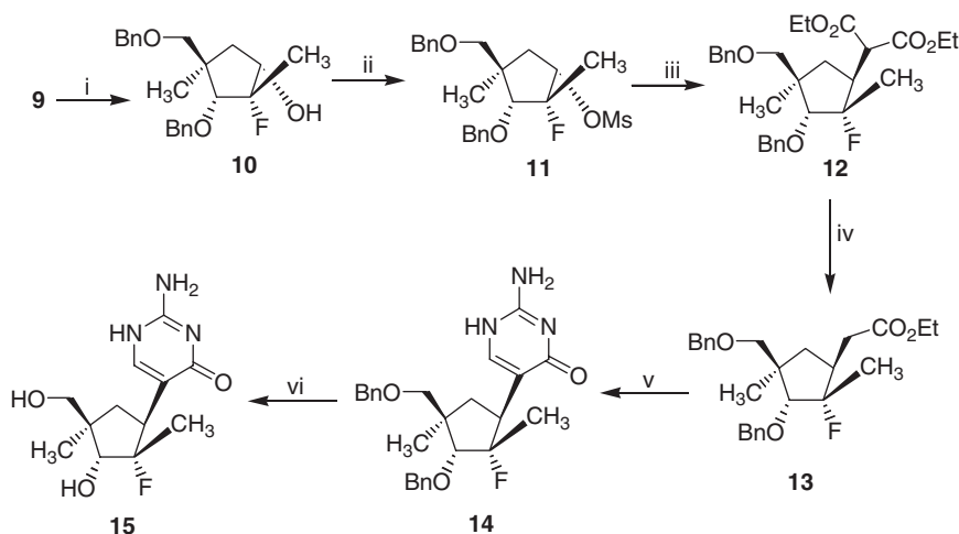
SCHEME 2 Synthesis of target 2'-fluorinated isocytosine nucleoside analogue. Reagents: i) 47% HF, (\text{NH}_4)_2\text{SiF}_6 , CsF; ii) MsCl, TEA, \text{CH}_2\text{Cl}_2 ; iii) NaH, \text{CH}_2(\text{CO}_2\text{Et})_2 , THF; iv) LiCl, DMSO; v) (a) LDA/THF, HCOEt; (b) \text{H}_2\text{NC}(=\text{NH})\text{NH}_2 .carbonate, NaOEt/EtOH; vi) Pd black, 5% \text{HCO}_2\text{H} in MeOH, reflux overnight.
