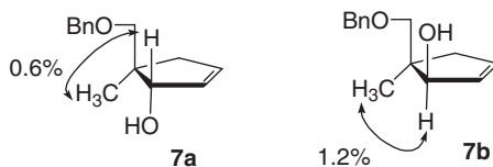
FIGURE 2 NOE differences of isomers 7a & 7b .
